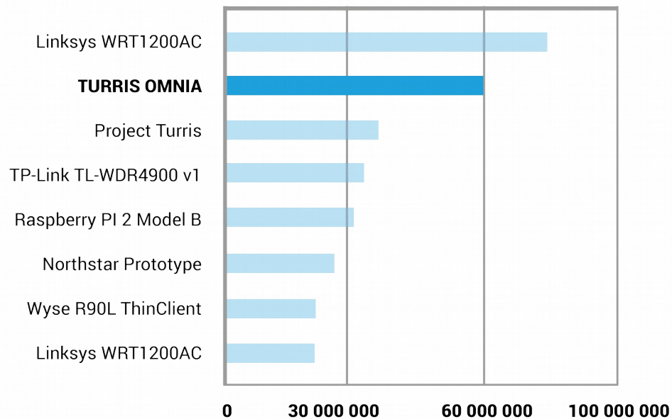
AES-128 benchmark
